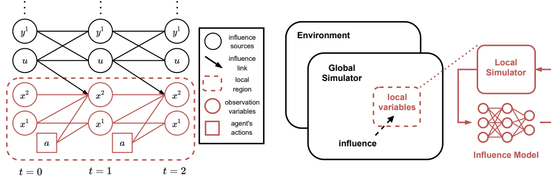
Figure 1. Left: A Dynamic Bayesian Network of a Local-POMDP unrolled 3 timesteps. Right: A diagram of the IALS.
