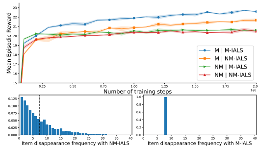
Figure 6. Top: Learning curves of agents with (M) and without memory (NM) trained on M-IALS and NM-IALS. Bottom: item disappearance frequencies with NM-IALS and with M-IALS.
