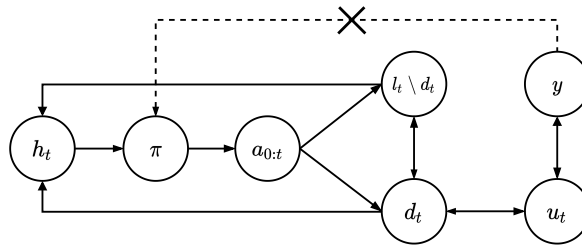
Figure 7. Graphical causal model of a local POMDP. The bidirectional arrows between two sets of variables (e.g. between d_t and u_t ) indicate that there can be variables in one set that are affected by other variables in the other set and vice-versa. As depicted by the two diagonal arrows in the middle, actions a_{0:t} may or may not be included in d_t . The top dashed arrow connecting y and \pi indicates that \pi cannot be a function of the non-local variables.
