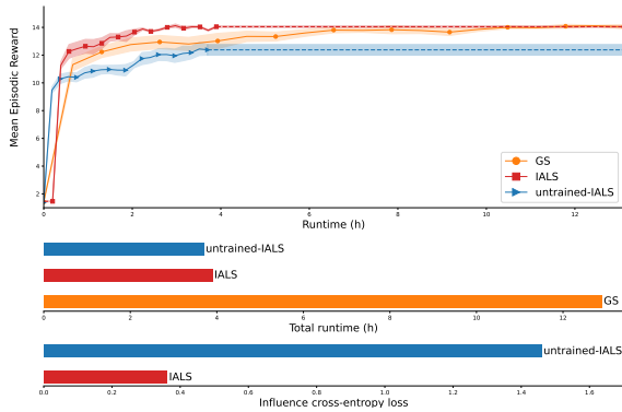
Figure 5. Top: Learning curves of agents trained with the GS, the IALS and the untrained-IALS on the the warehouse environment as a function of wall-clock time. Middle: Total runtime of training for 2M steps on the three simulators. Bottom: Cross entropy loss for the trained and untrained AIPs.
