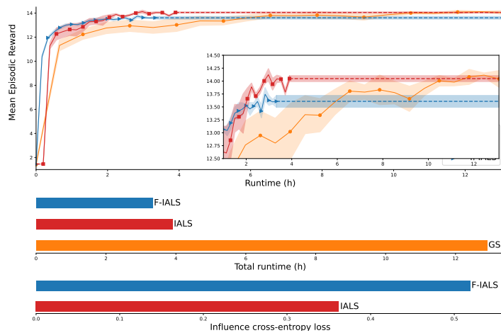
Figure 12. Top: Learning curves of agents trained with the GS, the IALS and the F-IALS on the the warehouse commissioning task as a function of wall-clock time. Zoom in version of the same chart showing the performance difference between IALS and F-IALS. The dotted horizontal lines show the final performance of the agents after 2M timesteps of training. The dotted horizontal line at the beginning of the red curve corresponds to the AIP training time. Second from the bottom: Total runtime of training for 2M steps on the three simulators. Bottom: Cross entropy loss for the two AIPs.
