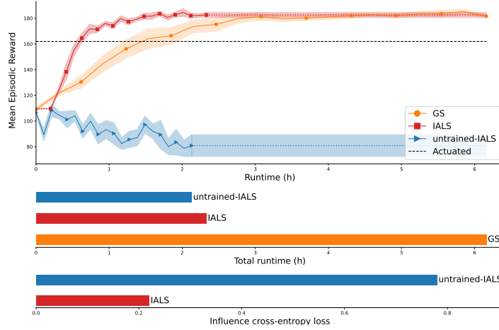
Figure 10. Top: Learning curves of agents trained with the GS, the IALS and the untrained-IALS on intersection 2 (Figure 2) as a function of wall-clock time. The dotted horizontal lines show the final performance of the agents after 2M timesteps of training. The dotted horizontal line at the beginning of the red curve corresponds to the AIP training time. Middle: Total runtime of training for 2M training steps on the three simulators. Bottom: Cross entropy loss for the trained and untrained AIPs.
