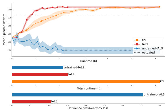
Figure 3. Top: Learning curves of agents trained with the GS, the IALS and the untrained-IALS on intersection 1 (Figure 2) as a function of wall-clock time. Middle: Total runtime of training for 2M training steps on the three simulators. Bottom: Cross entropy loss for the trained and untrained AIPs.
