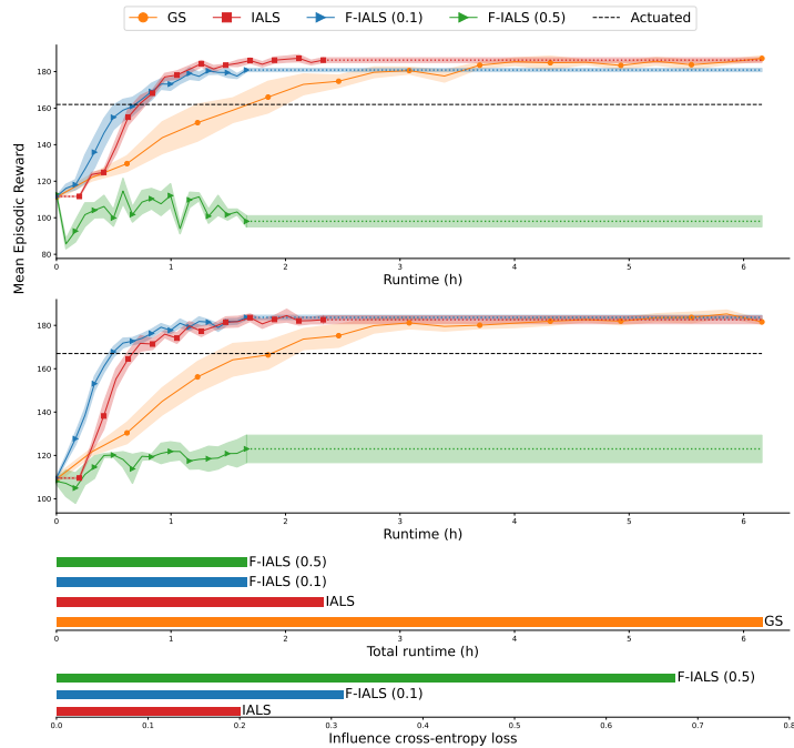
Figure 11. Top: Learning curves of agents trained with the GS, the IALS and the F-IALS on the the two intersections highlighted in Figure 2 as a function of wall-clock time. The dotted horizontal lines show the final performance of the agents after 2M timesteps of training. The short horizontal line at the beginning of the red curve corresponds to the AIP training time. Second from the bottom: Total runtime of training for 2M training steps on the three simulators. Bottom: Cross entropy loss evaluated at intersection 1 for the three AIPs (values are very similar for intersection 2).
