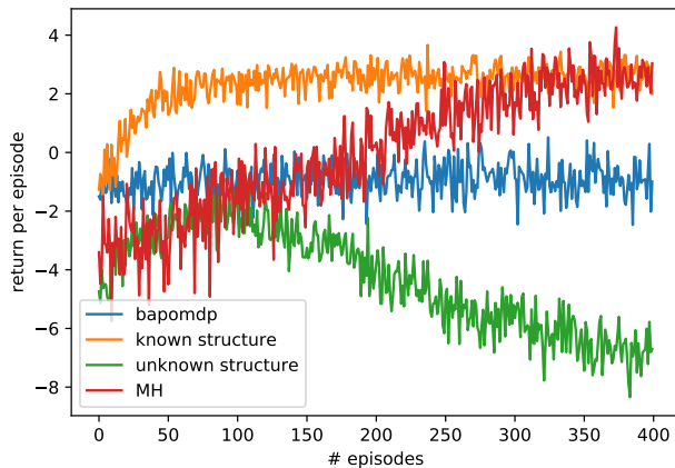
Figure 3: Average return on the Tiger problem
